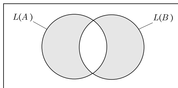
FIGURE 4.6 The symmetric difference of L(A) and L(B)
