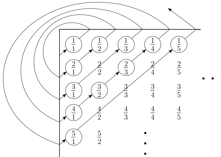
FIGURE 4.16 A correspondence of \mathcal{N} and \mathcal{Q} ■
